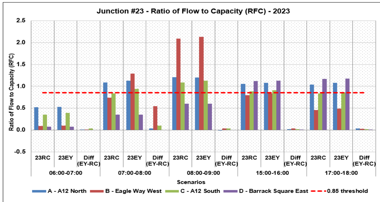
Plate 9.80: A12 / Eagle Way / Barrack Square Roundabout 2023 Early Years RFC Results
