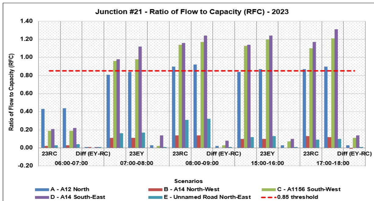
Plate 9.56: A12 / A14 Roundabout 2023 Early Years RFC Results
