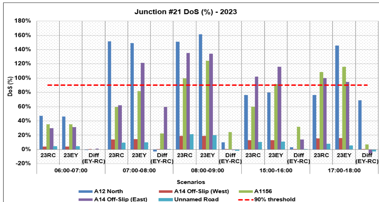
Plate 9.59: A12 / A14 Roundabout Mitigated 2023 Early Years Degree of Saturation (DoS) Results
