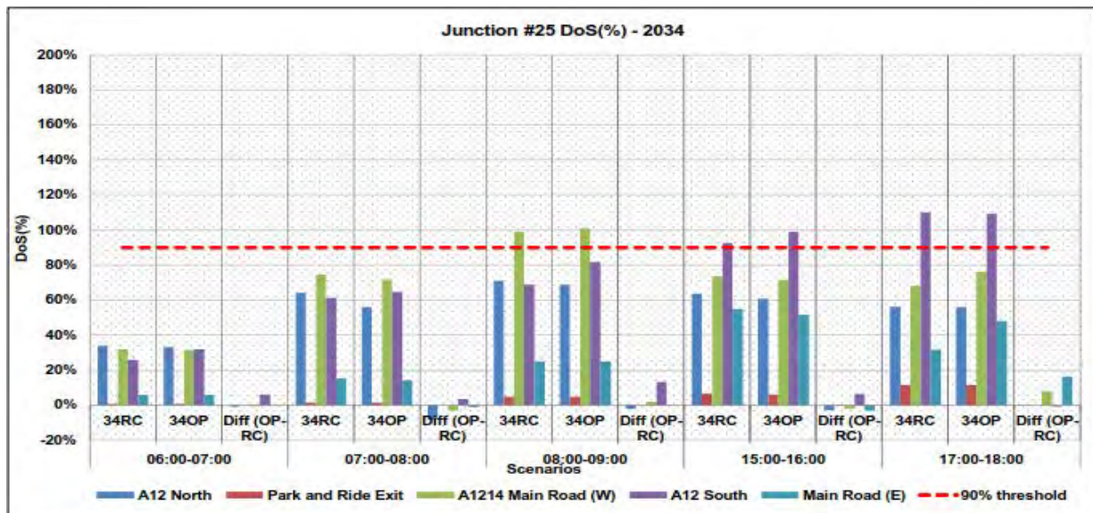
Plate 9.103: A12 / A1214 / Main Road / Martlesham Park and Ride Roundabout 2034 Sensitivity Test DOS Results
