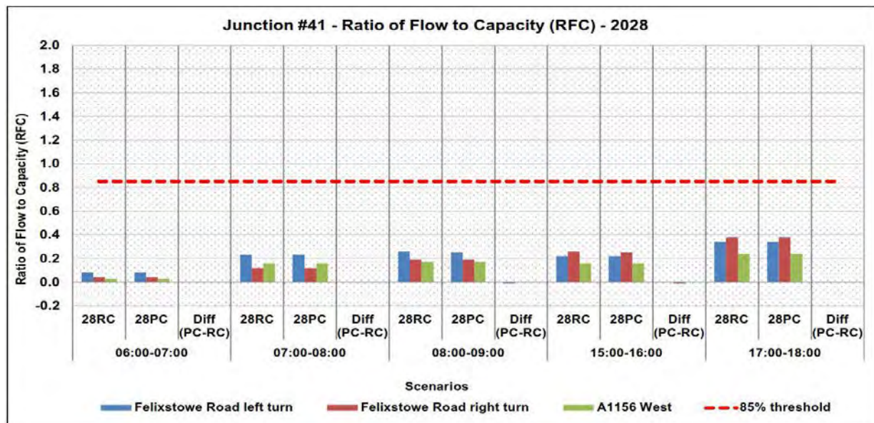
Plate 9.139: A1156 / Felixstowe Road T-Junction 2028 Peak Construction RFC Results
