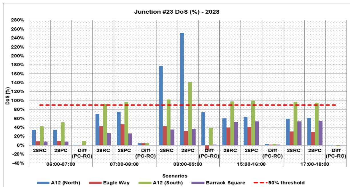
Plate 9.83: A12 / Eagle Way / Barrack Square Roundabout Mitigated 2028 Peak Construction RFC Results
