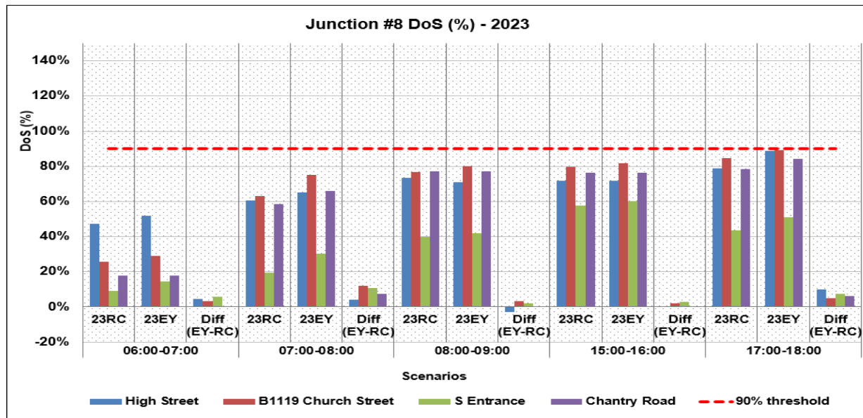
Plate 9.33: B1121 / B1119 Saxmundham Crossroads 2023 Early Years Degree of Saturation Results
