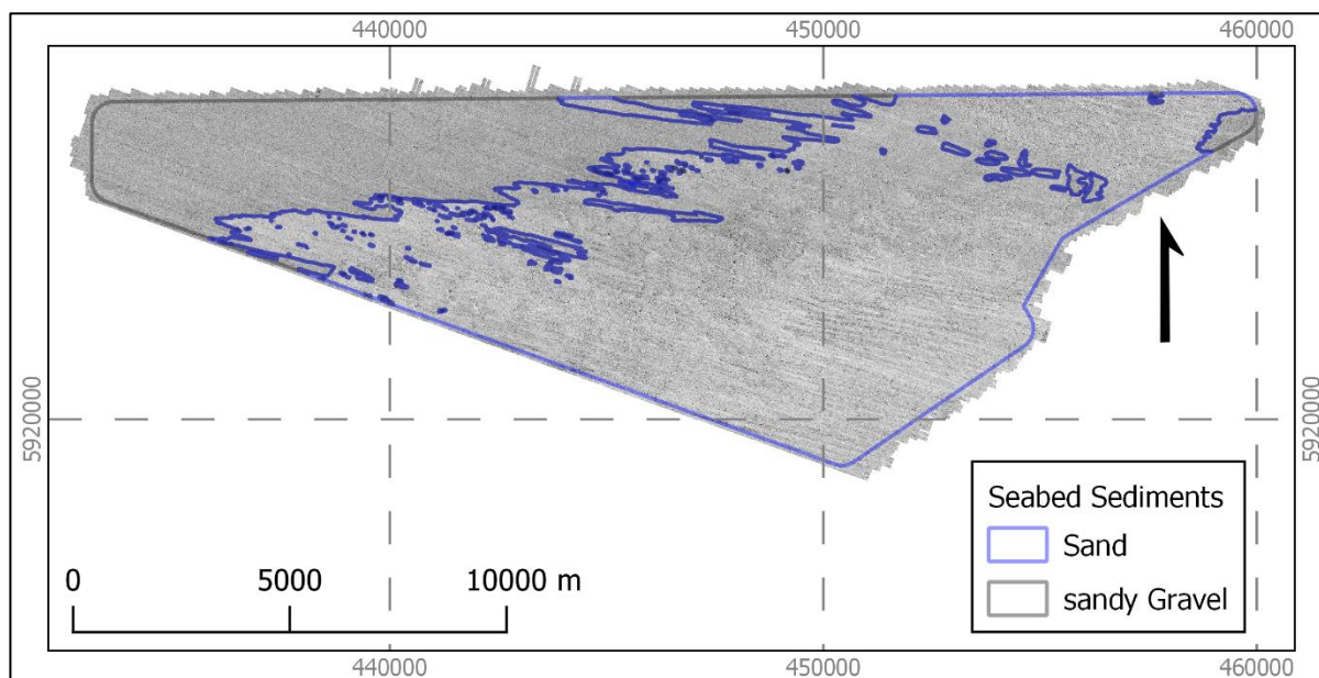
Figure 4.5: Side Scan Sonar example of the seafloor sediments interpretation
