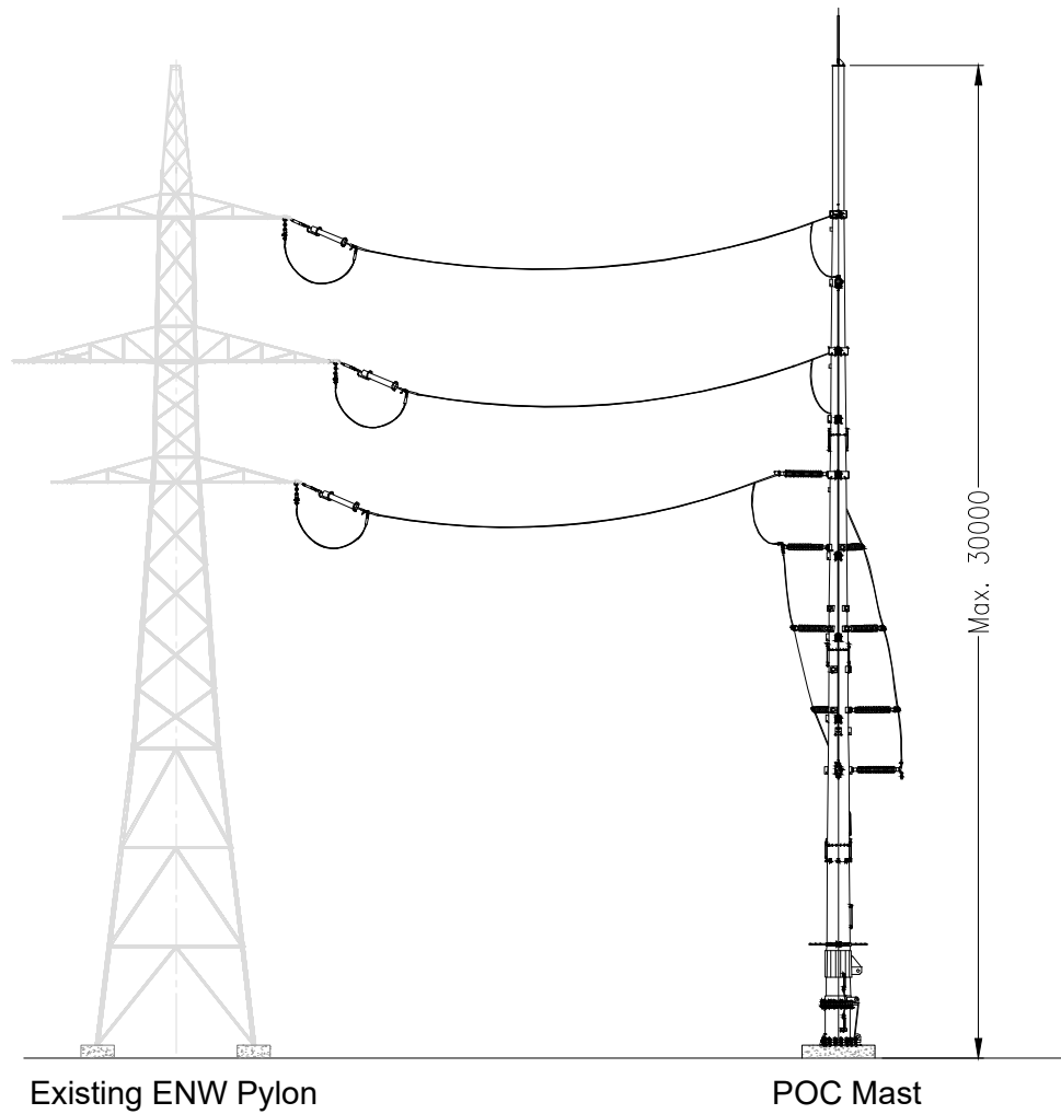
FRONT VIEW
