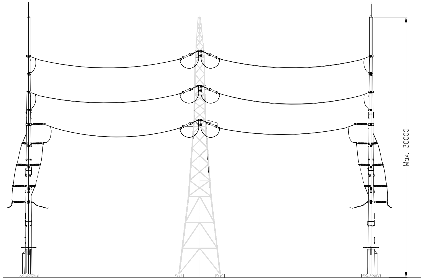
SIDE VIEW
