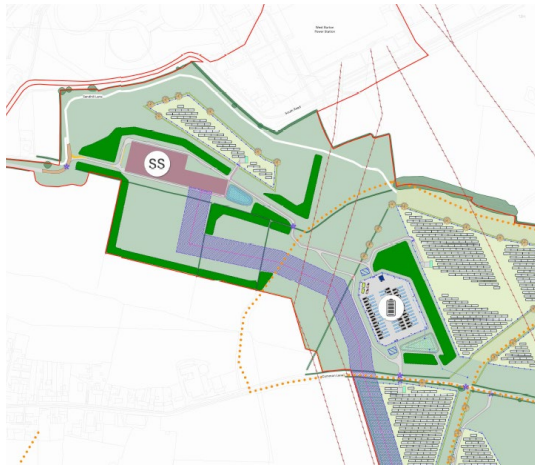
Figure 15.7 -- Onsite Substation and BESS Compound Extract from Figure 2.1 – Indicative Site Layout [EN010163/APP/6.4.1]
