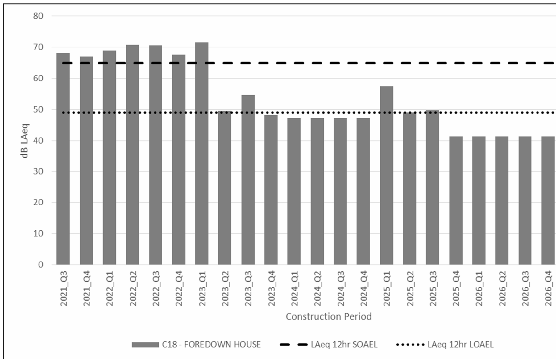
Figure 2-18 C18 Foredown House Predicted Construction Noise Levels
