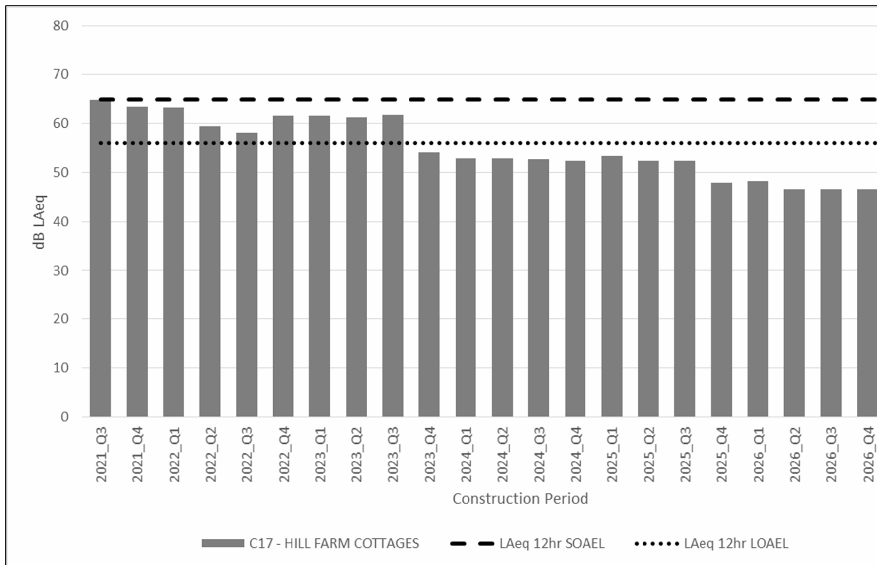
Figure 2-17a C17 Hill Farm Cottages Predicted Daytime Construction Noise Levels
