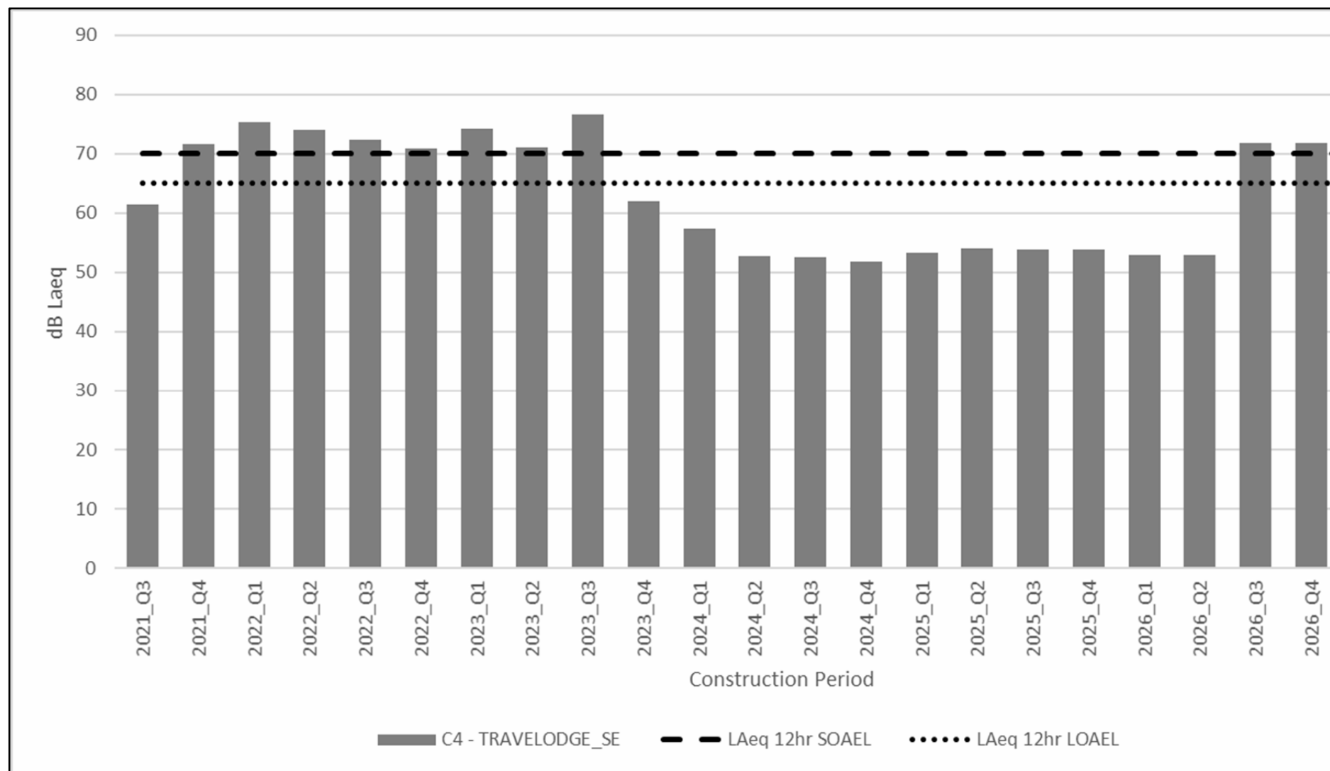
Figure 2-4 C4 Travelodge (SE facade) Predicted Construction Noise Levels
