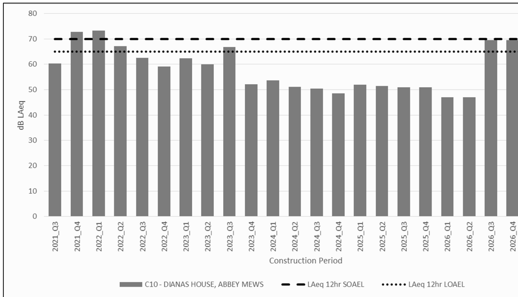
Figure 2-10 C10 Diana's House, Abbey Mews Predicted Construction Noise Levels
