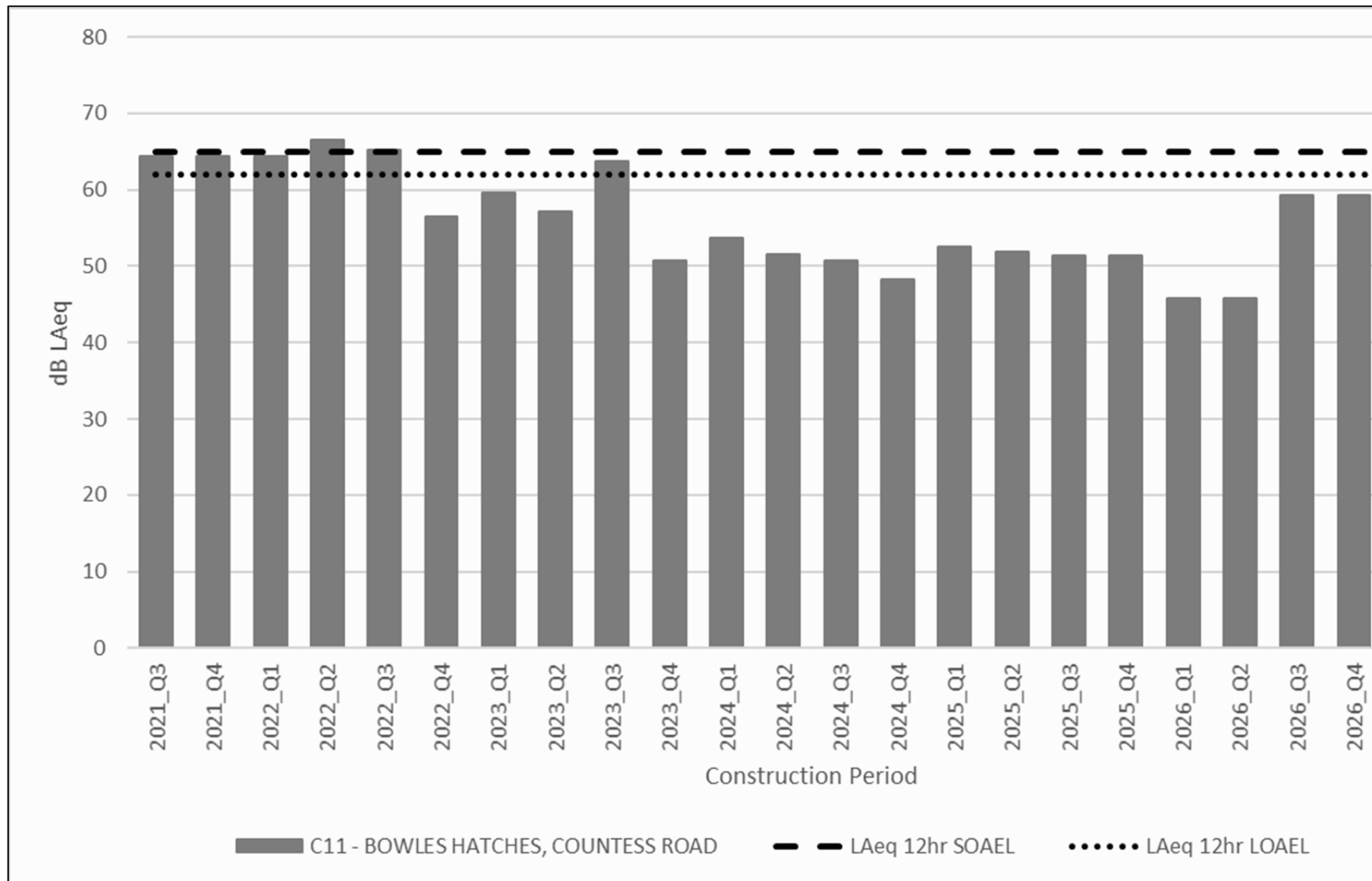
Figure 2-11 C11 Bowles Hatches, Countess Road Predicted Construction Noise Levels
