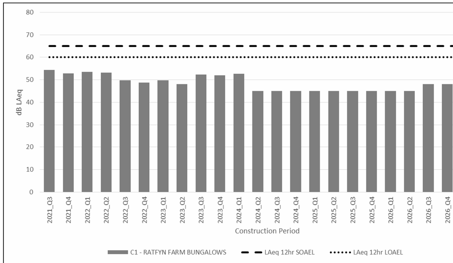
Figure 2-1 C1 Ratfyn Farm Bungalows Predicted Construction Noise Levels
