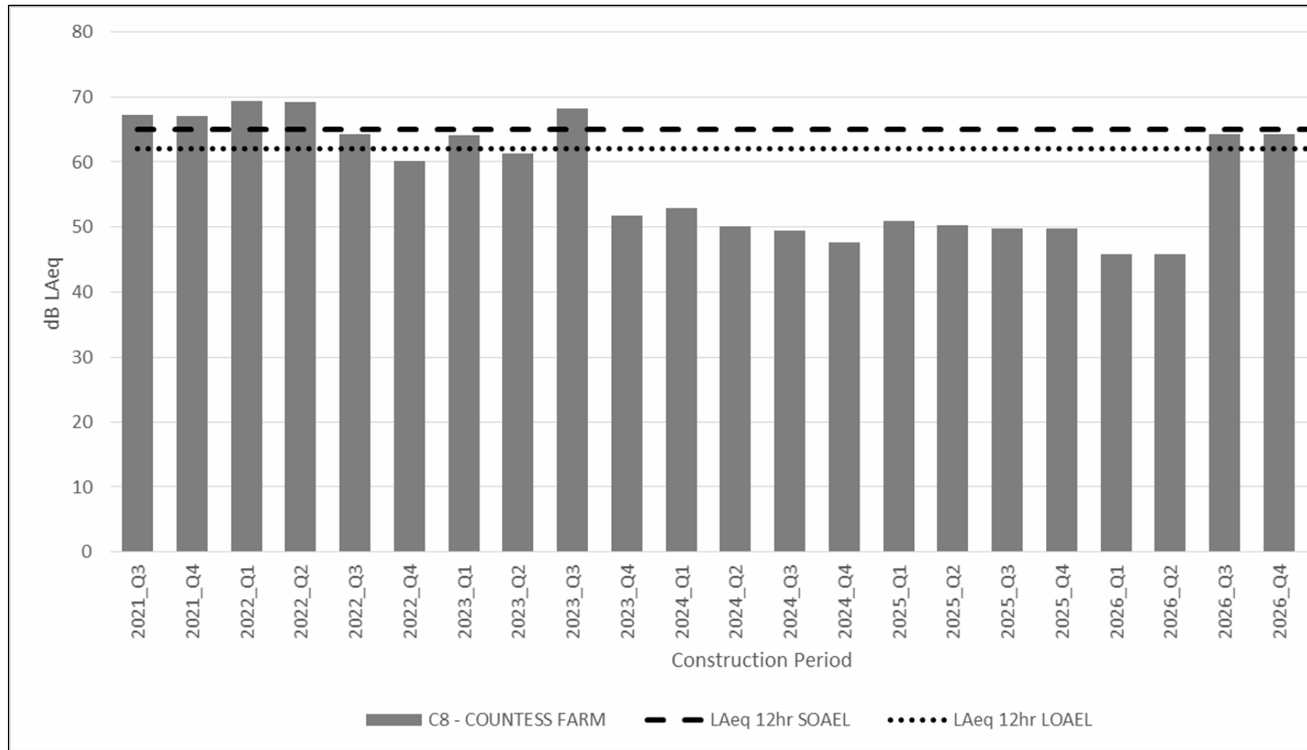
Figure 2-8 C8 Countess Farm Predicted Construction Noise Levels
