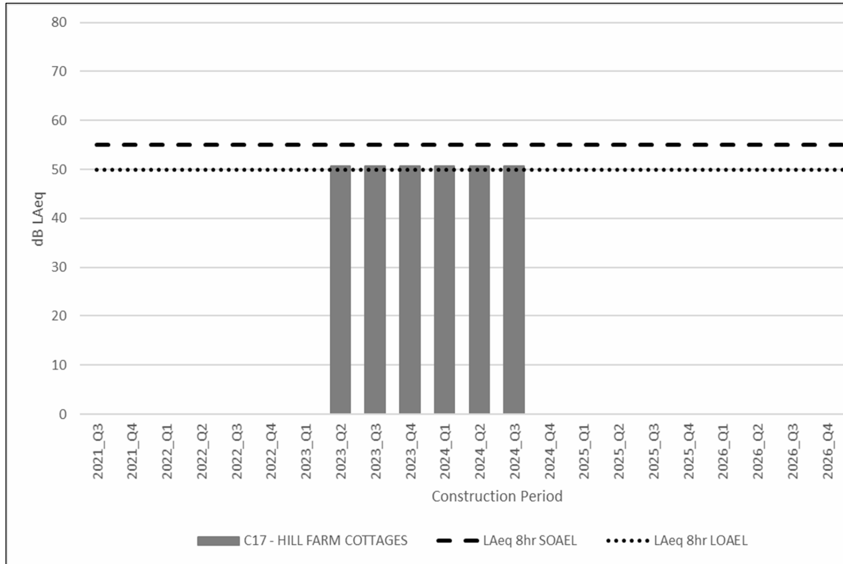
Figure 2-17b C17 Hill Farm Cottages Predicted Night-time Construction Noise Levels
