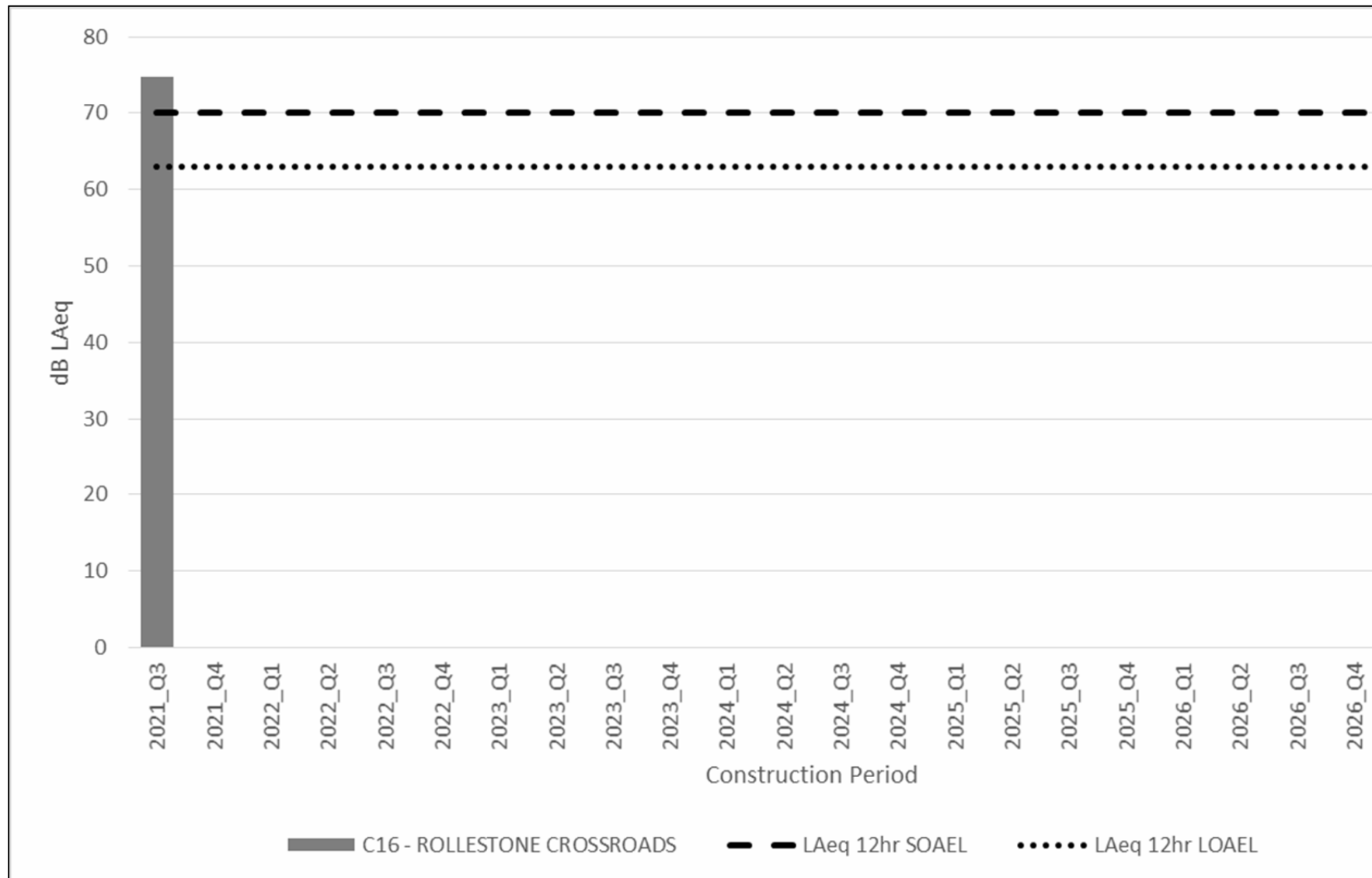
Figure 2-16 C16 Rolleston Crossroads Predicted Construction Noise Levels
