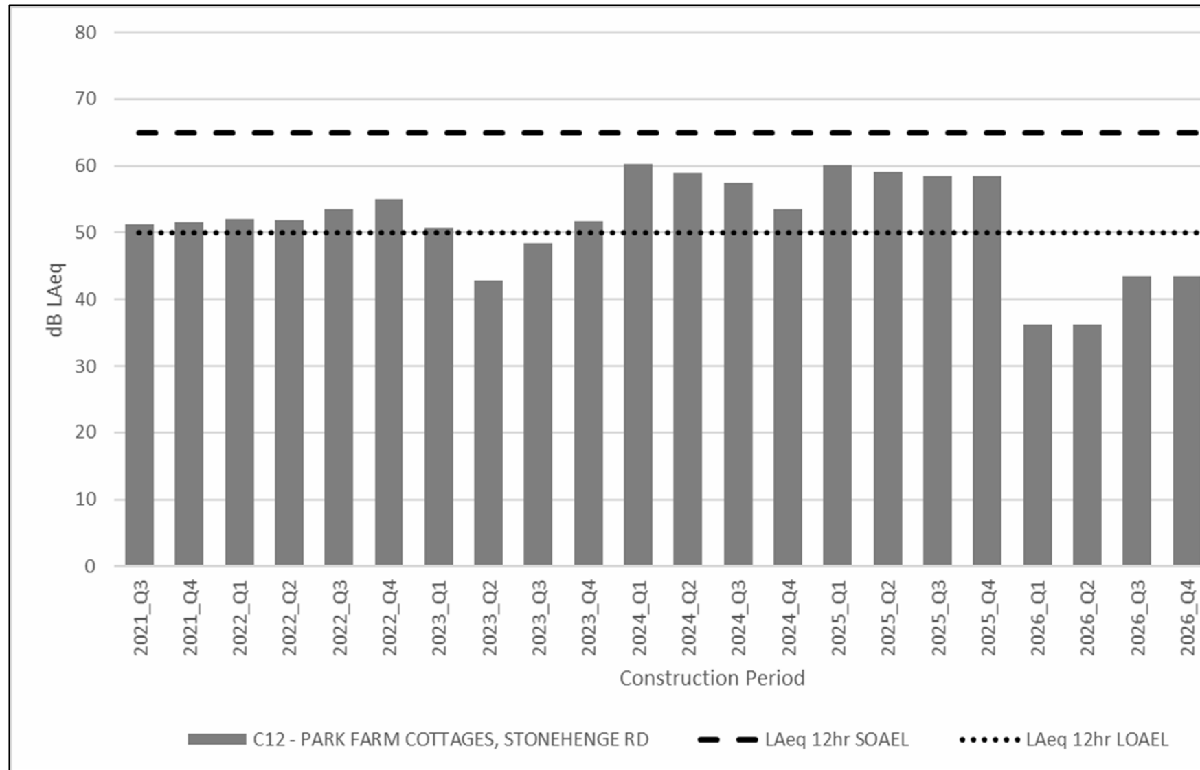
Figure 2-12 C12 Park Farm Cottages Predicted Construction Noise Levels
