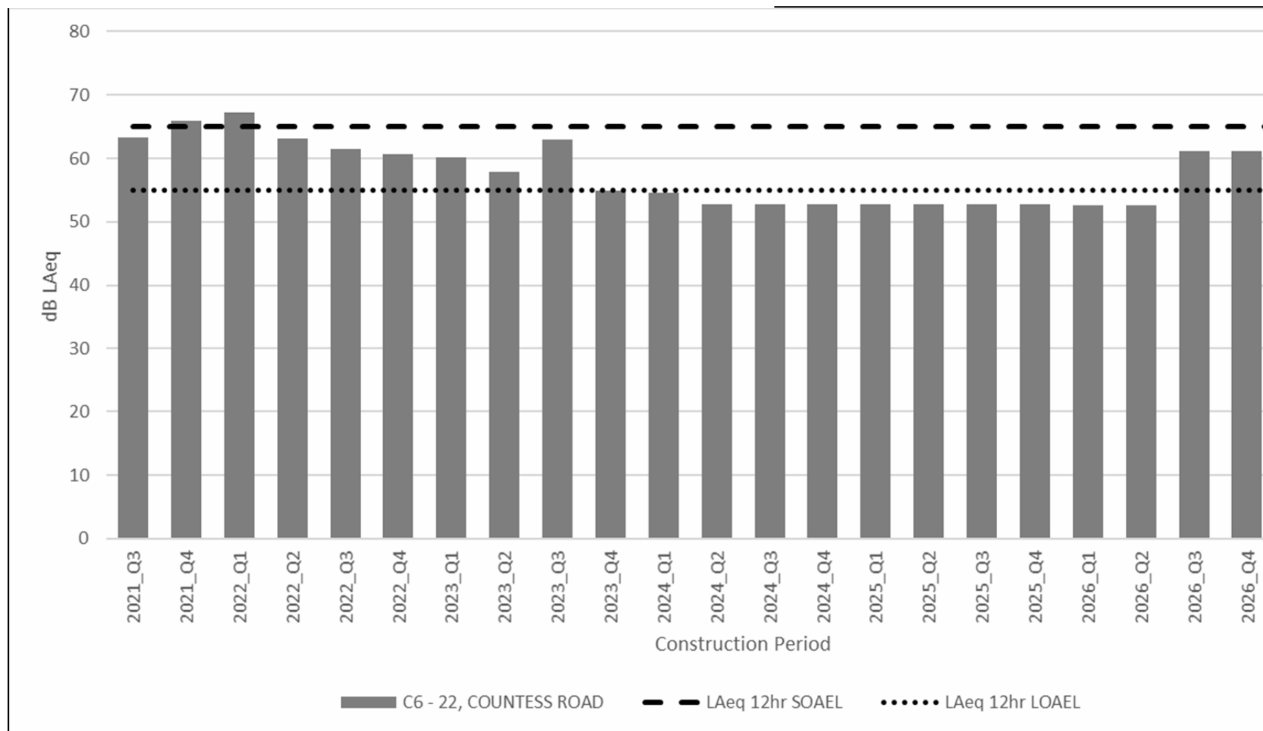
Figure 2-6 C6 22 Countess Road Predicted Construction Noise Levels
