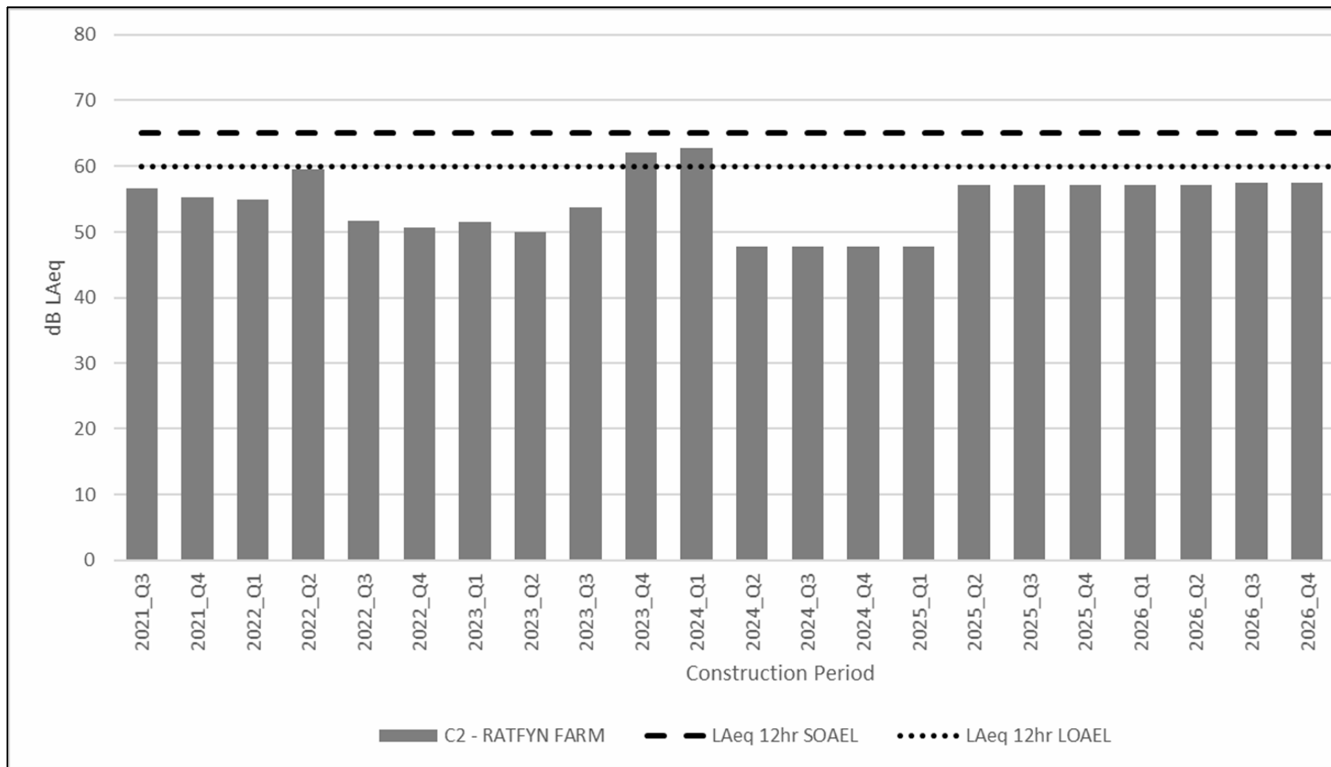
Figure 2-2 C2 Ratfyn Farm Predicted Construction Noise Levels
