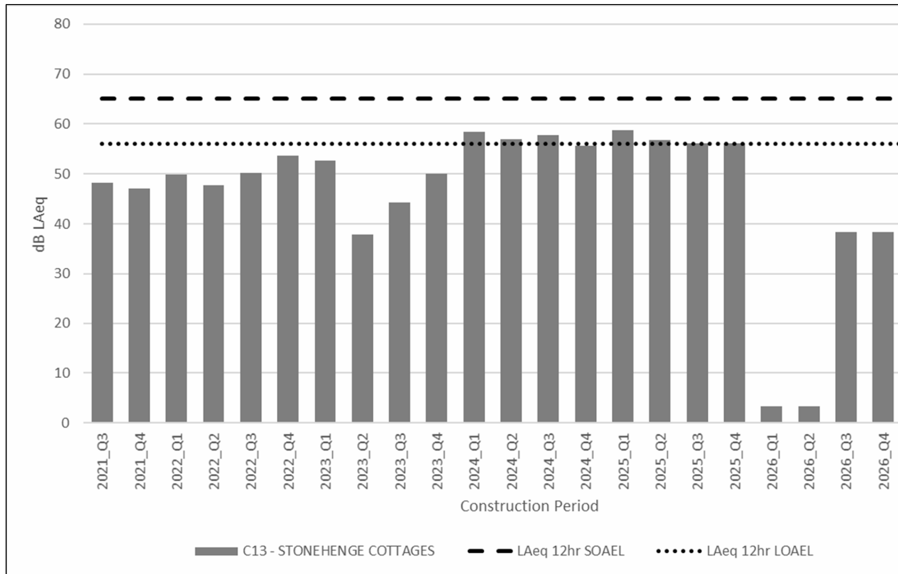
Figure 2-13 C13 Stonehenge Cottages Predicted Construction Noise Levels
