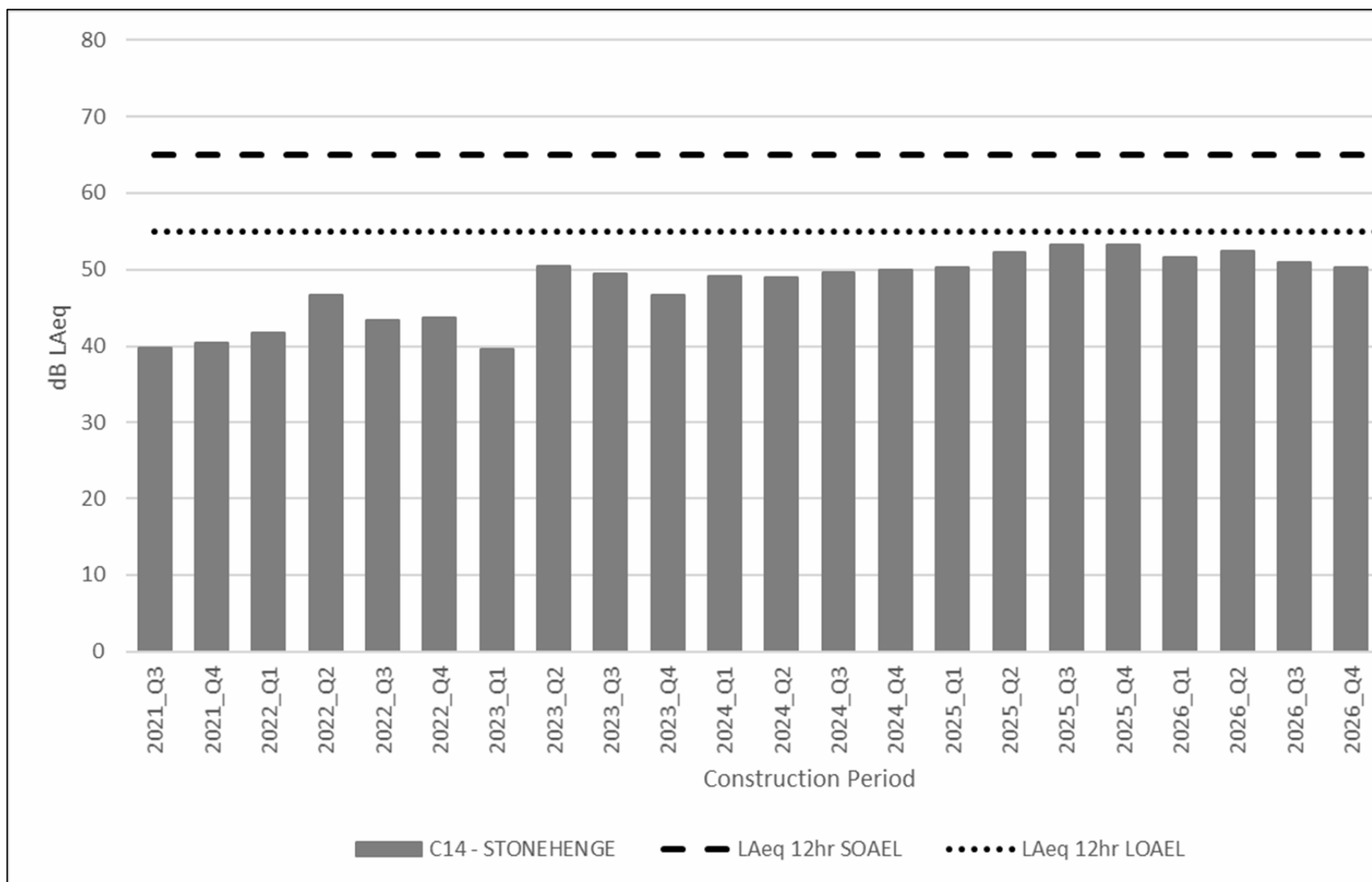
Figure 2-14 C14 Stonehenge Predicted Construction Noise Levels
