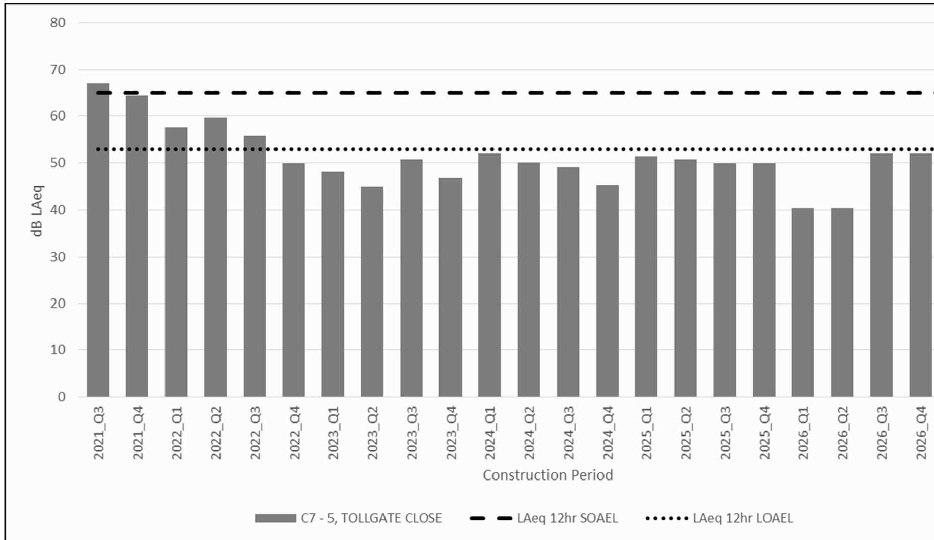
Figure 2-7 C7 5 Tollgate Close Predicted Construction Noise Levels
