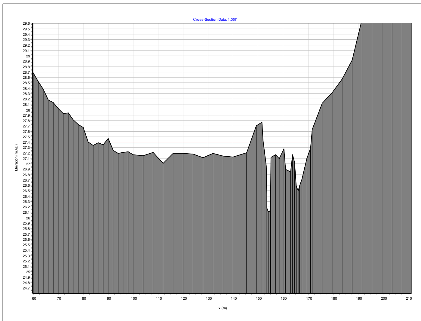
Figure 3: Cross section data showing out of bank flows
