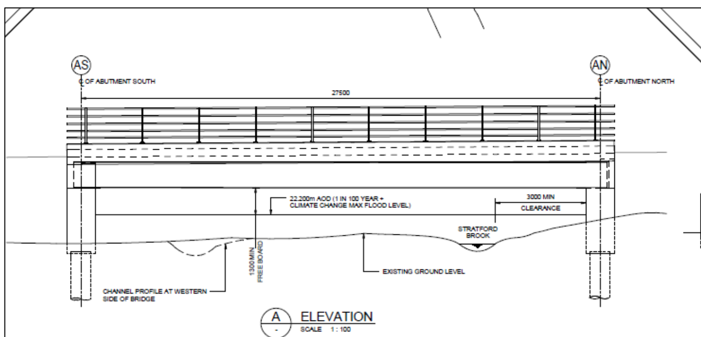
Figure 4: Extract from Bridge drawing
