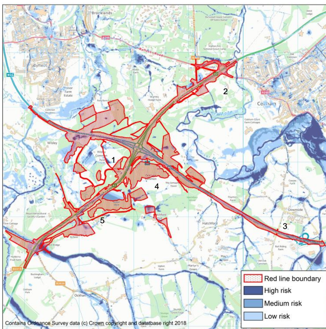
Figure 2.2: Environment Agency surface water mapping
