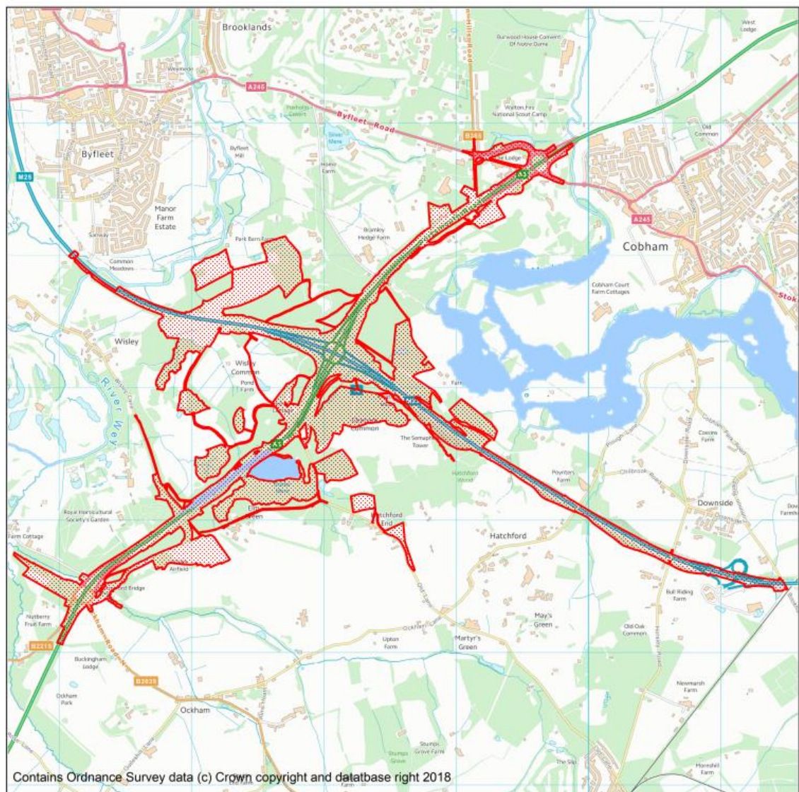
Figure 2.3: Environment Agency reservoir inundation mapping
