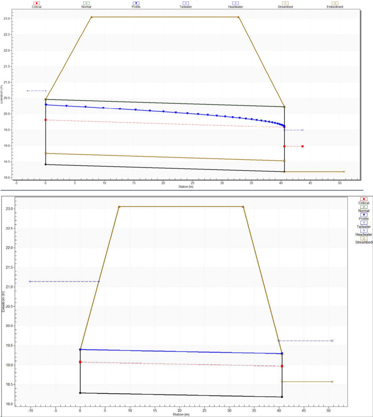
Figure 4-2: HY-8 A1 long section and 1 in 100-year plus 65% climate change event
