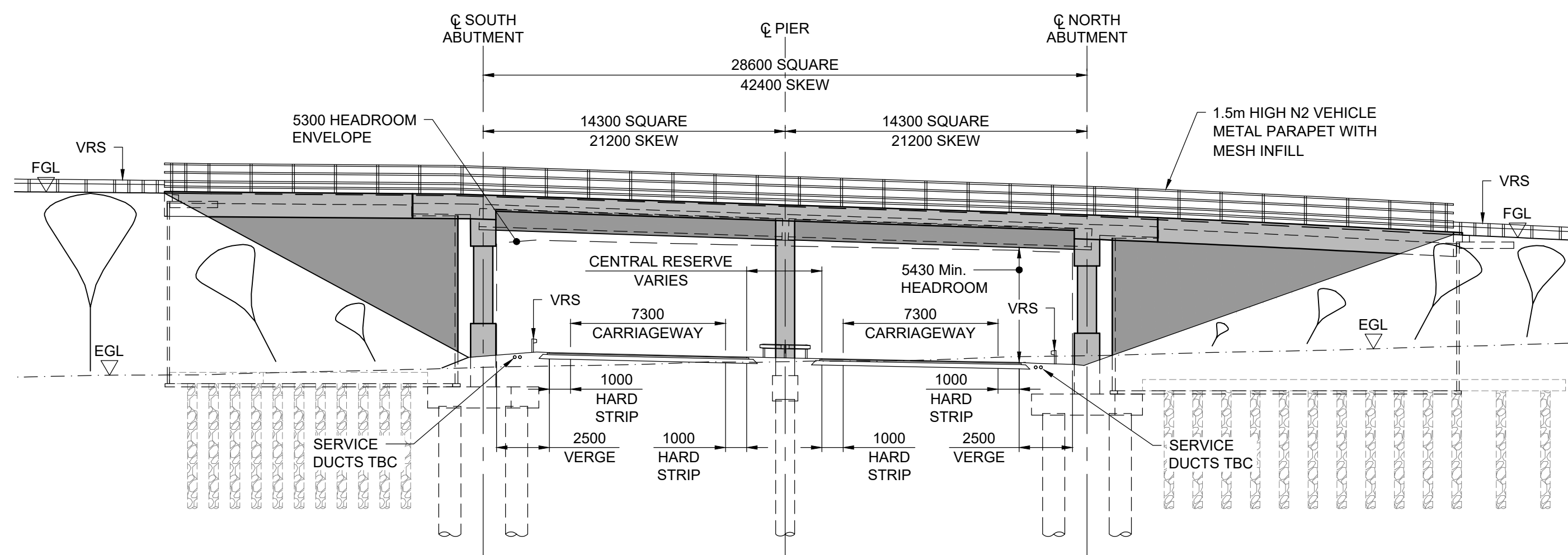
ELEVATION ON A SCALE 1:200
