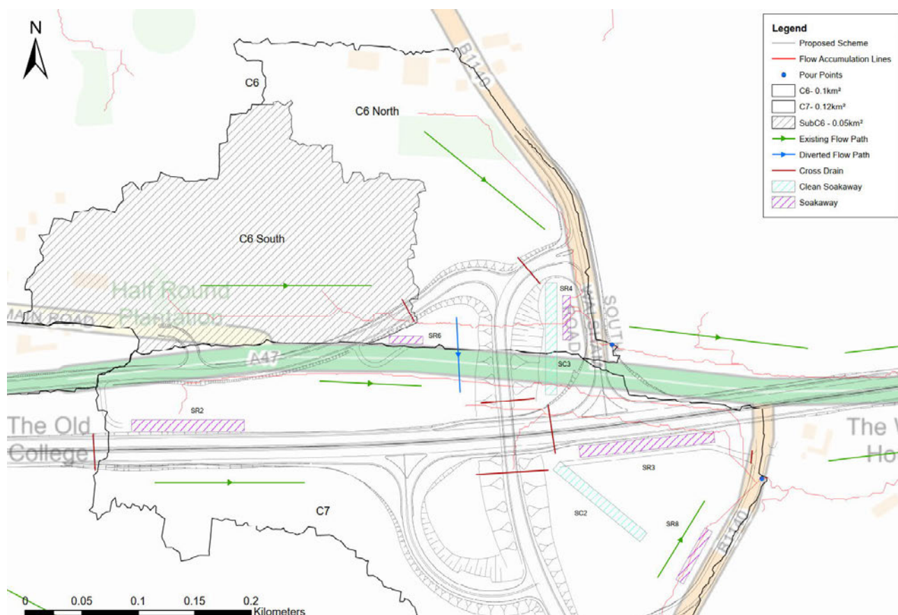
Figure 8-1 Natural catchment drainage around South Walsham Junction
