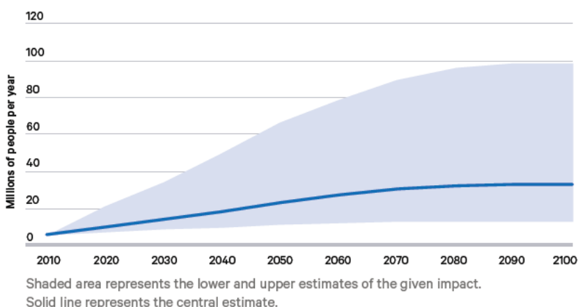
River flooding greater than the reference 50-year flood (assumes no additional flood defences)
