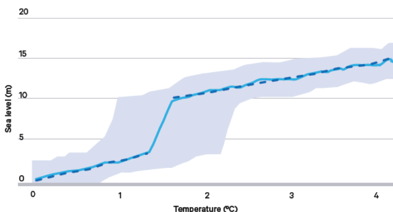
Committed sea level rise as a function of long-term global temperature increase
