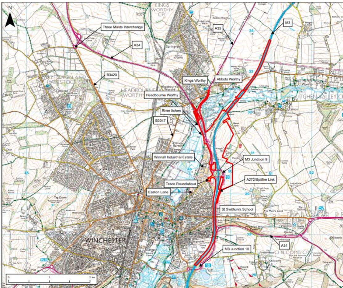
Figure 2-1: Application Boundary and Key Links (Source: Case for the Scheme Document Ref: 7.1)
