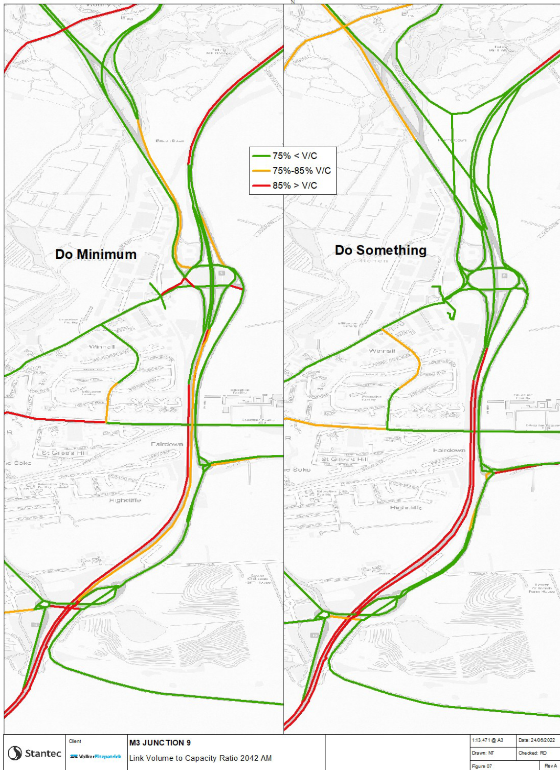
Figure 4-13: Volume to Capacity Ratio, 2042 Do-Something and Do-Minimum AM Peak
