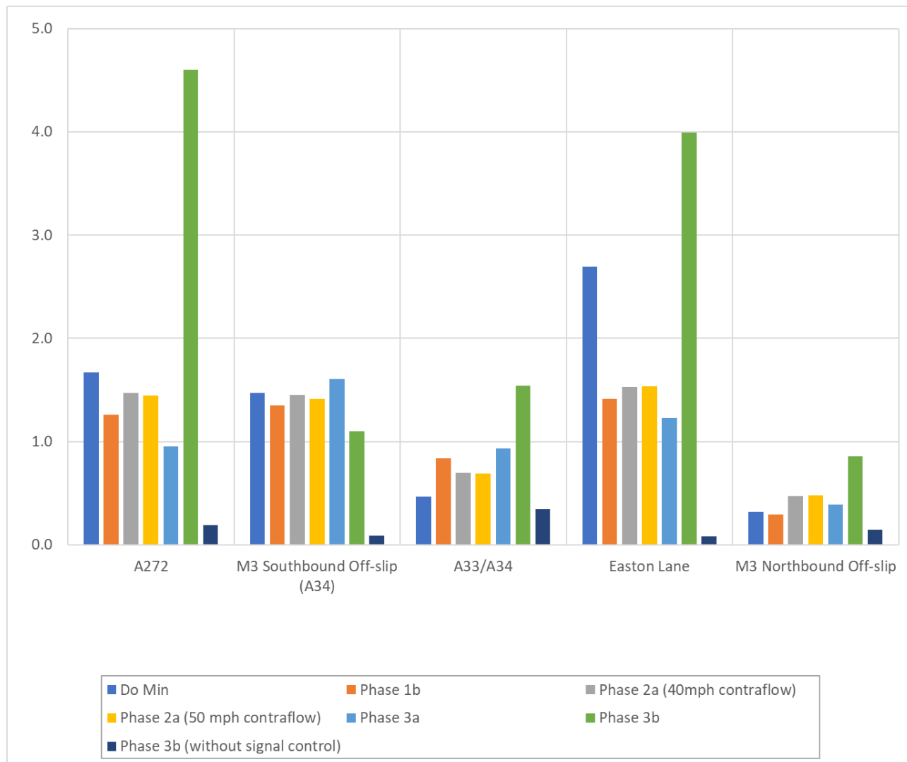
Figure 2.6: AM Peak Hour Modelled Delays (minutes)
