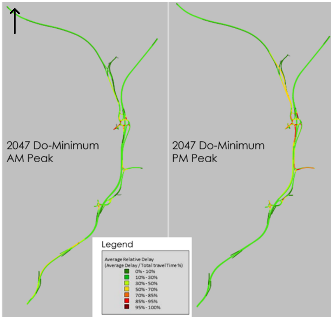
Figure 4-17: 2047 Do-Minimum Delay Heatmaps
