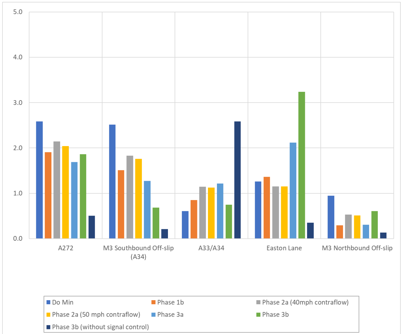
Figure 2.7: PM Peak Hour Modelled Delays (minutes)
