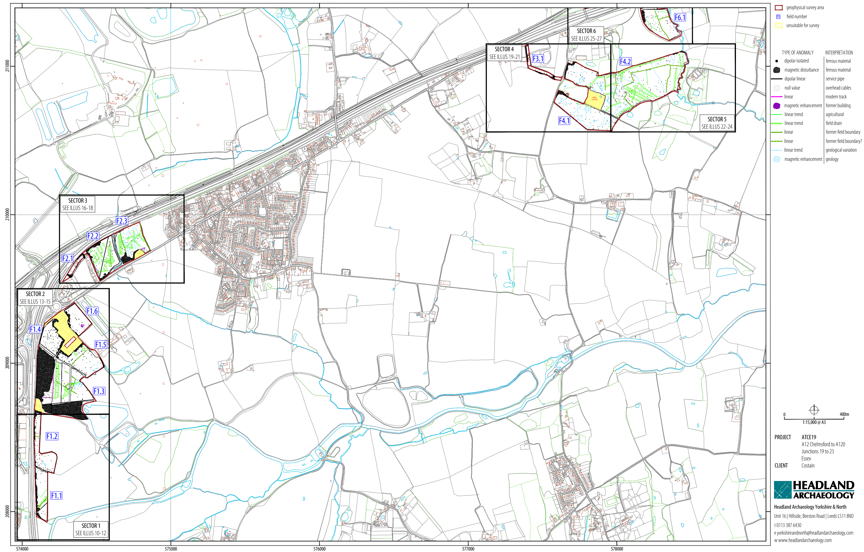
ILLUS 3 Overall interpretation plot of magnetometer data, West
