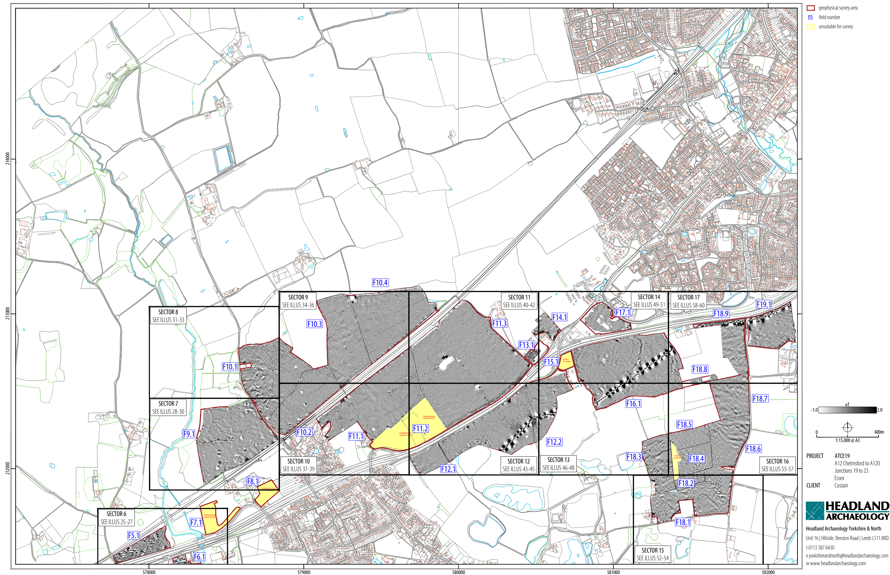
ILLUS 4 Overall greyscale plot of magnetometer data, Centre West
