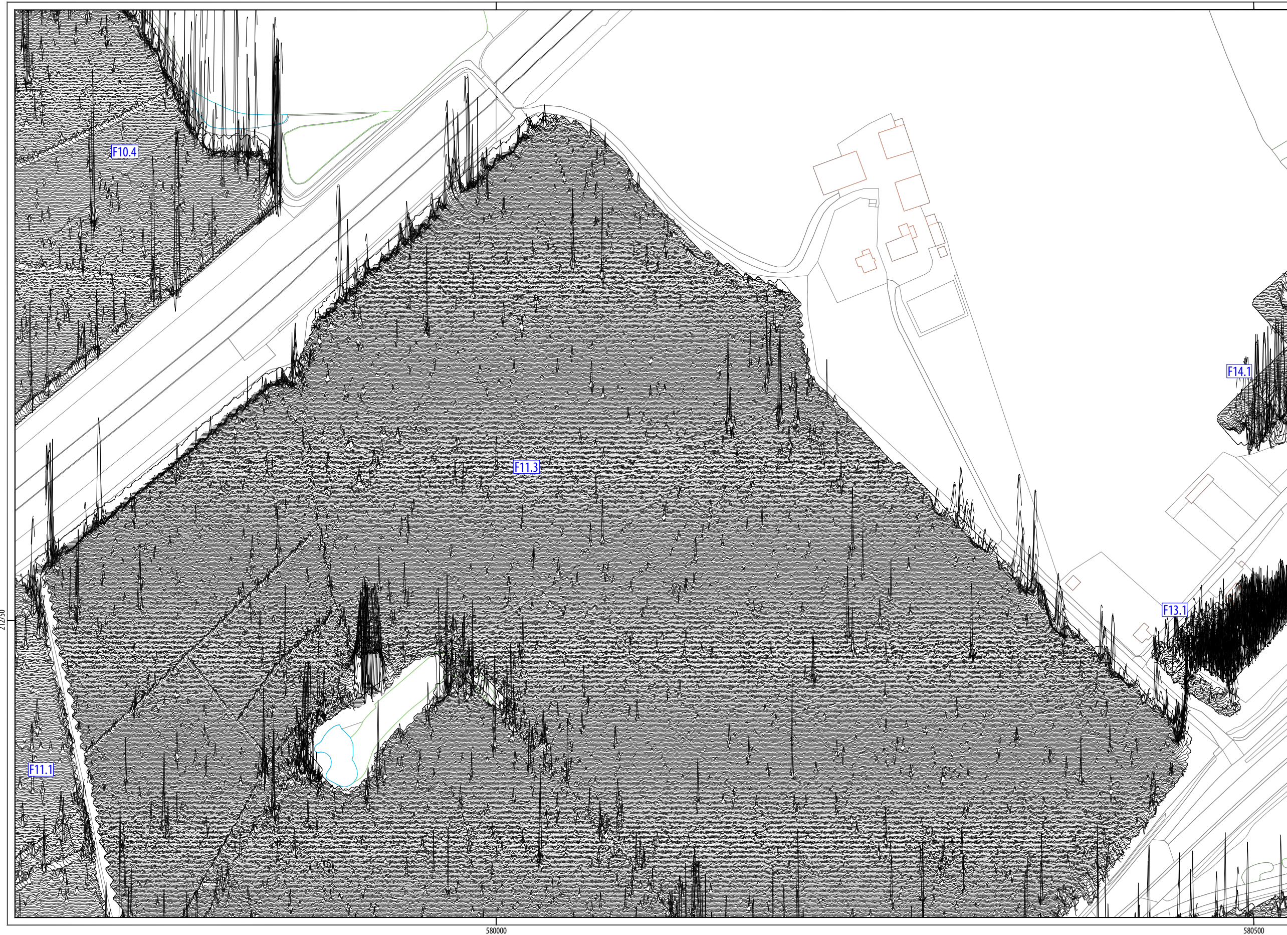
ILLUS 41 XY trace plot of minimally processed magnetometer data; Sector 11
