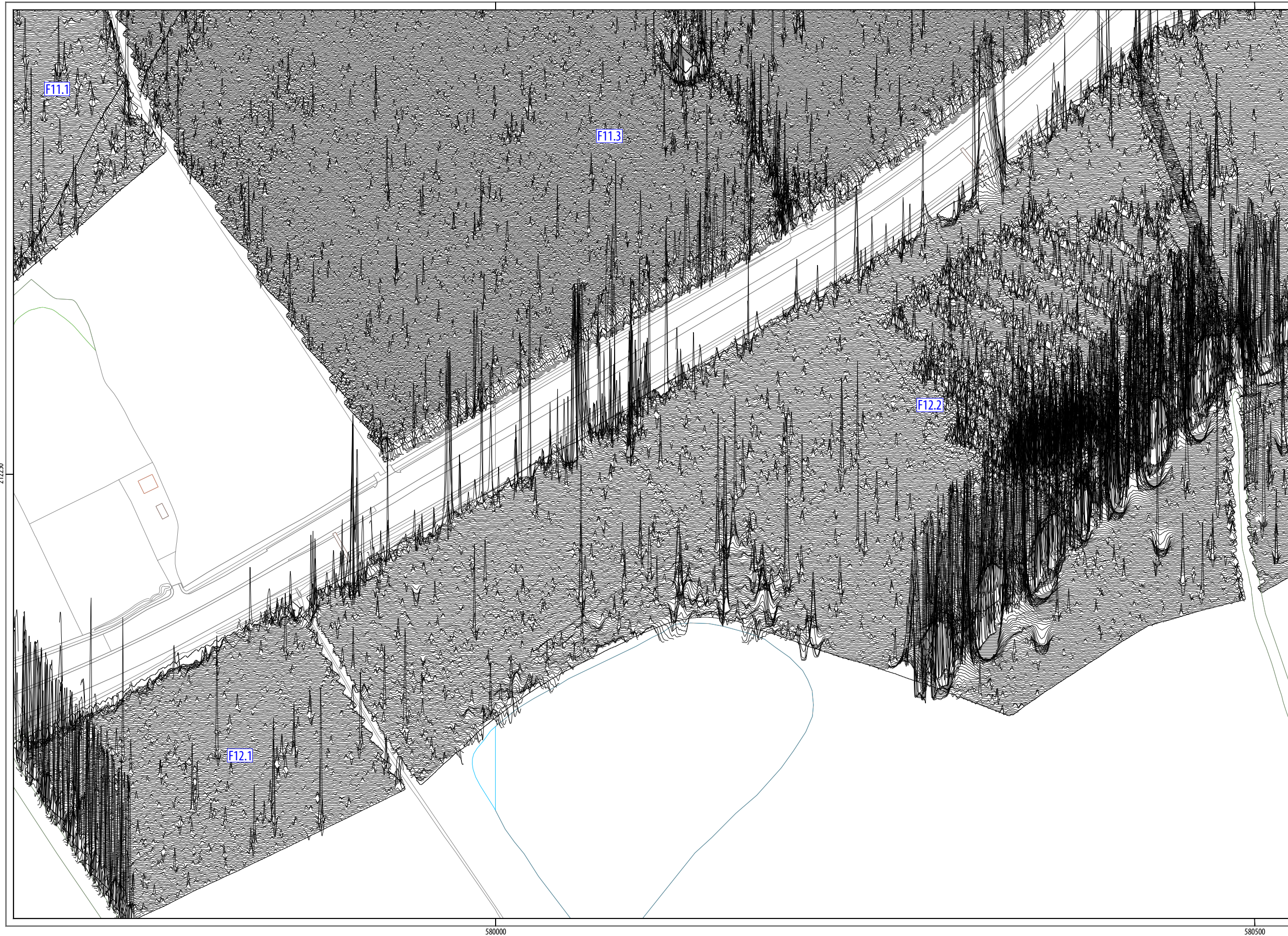
ILLUS 44 XY trace plot of minimally processed magnetometer data; Sector 12
