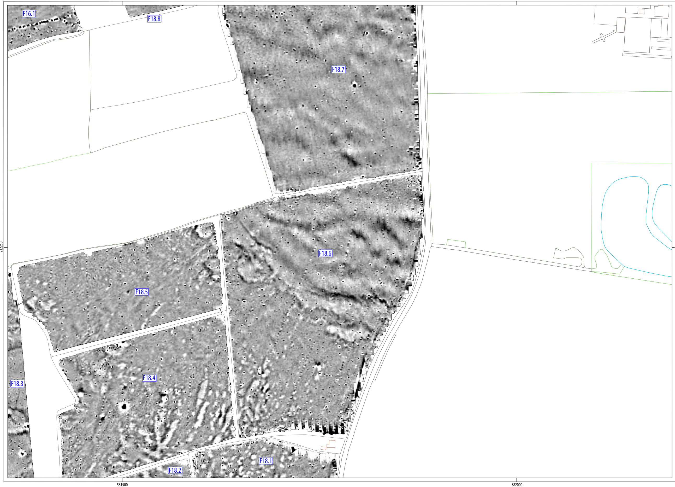
ILLUS 55 Processed greyscale magnetometer data; Sector 16
