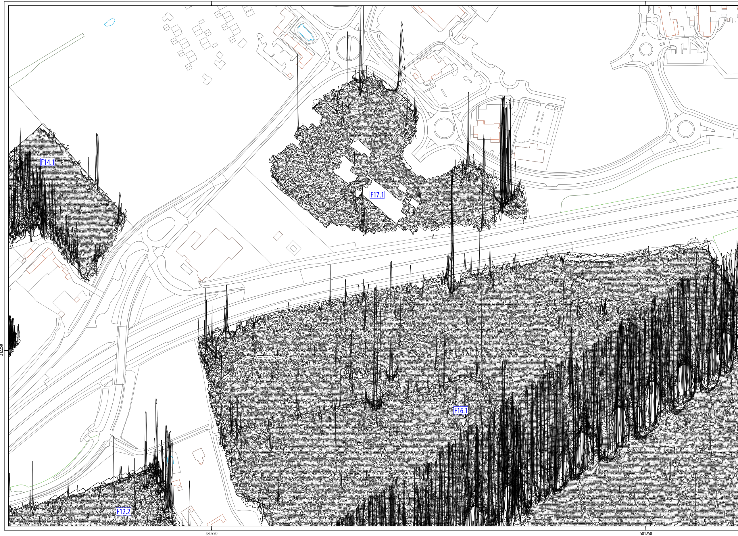
ILLUS 50 XY trace plot of minimally processed magnetometer data; Sector 14
