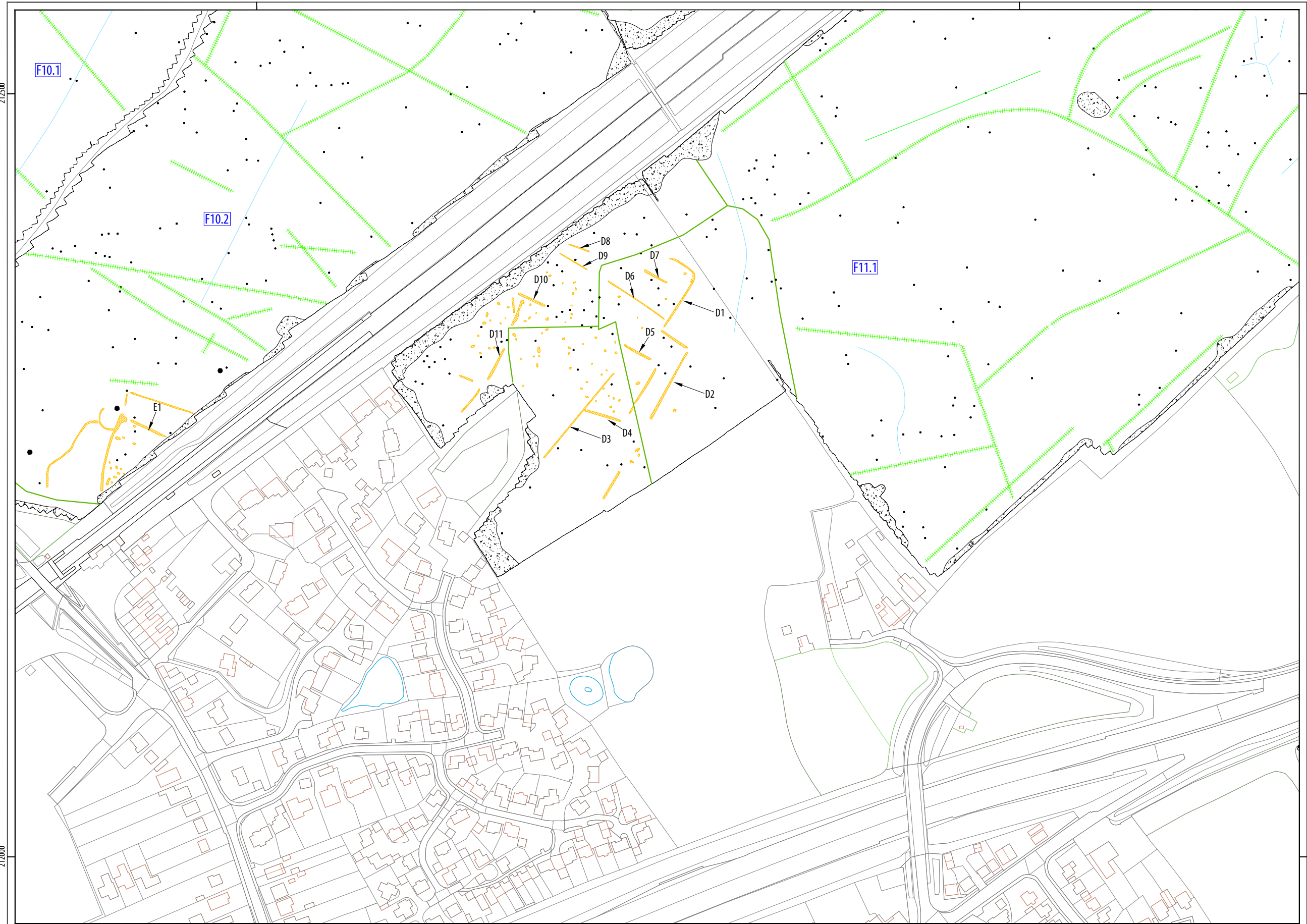
ILLUS 39 Interpretation of magnetometer data; Sector 10
