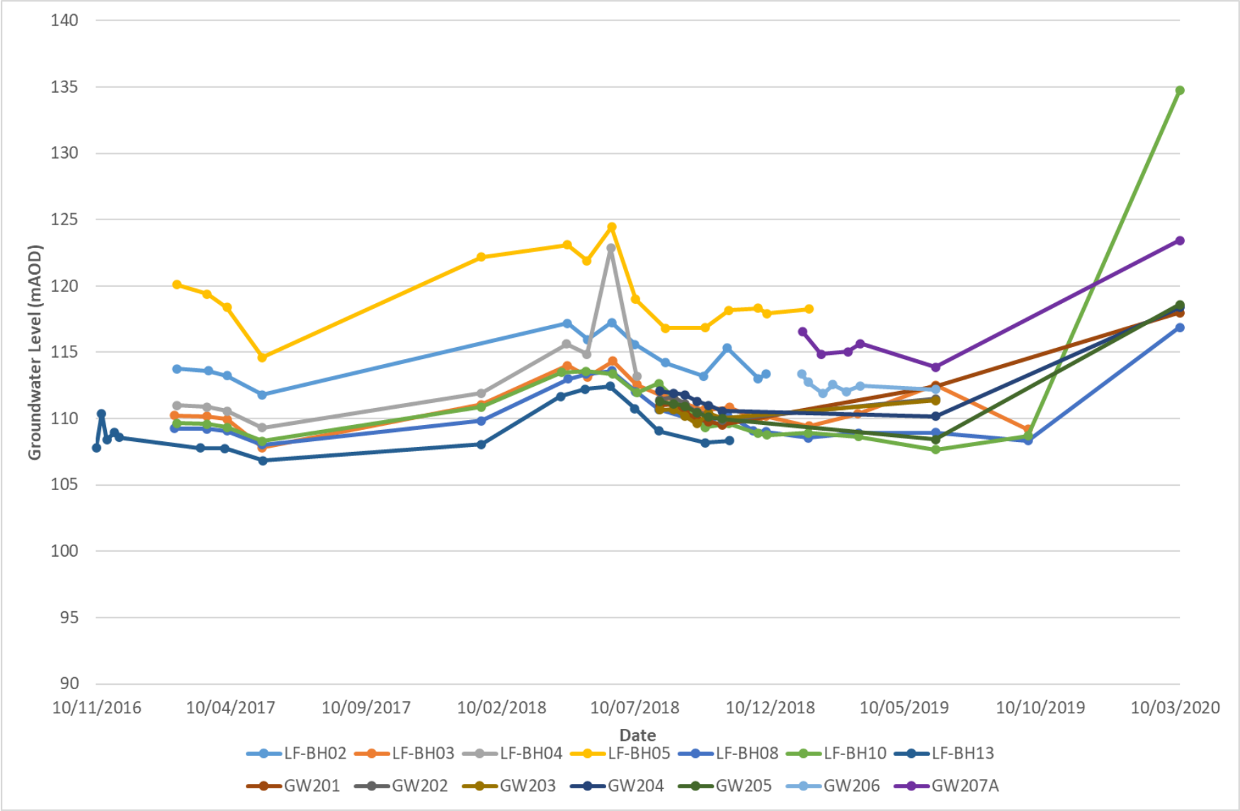
Figure 9 – Groundwater Hydrograph from Monitoring (Beneath WVG Landfill)
